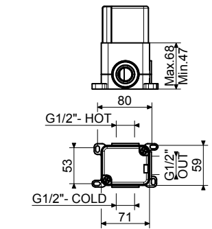
Scatola incasso Handy Box per miscelatore Ø35. Single-lever mixer for concealed installation, Ø 35 mm
