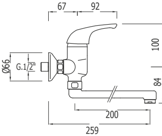
GEMMA Miscelatore lavello a parete con bocca girevole Wall mounted single lever sink mixer with swivel spout
