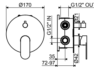
Miscelatore incasso con deviatore 2-3 uscite. Scatola incasso venduta separatamente Single-lever mixer for concealed installation, with 2-3 outlets. The built-in box is sold separately
